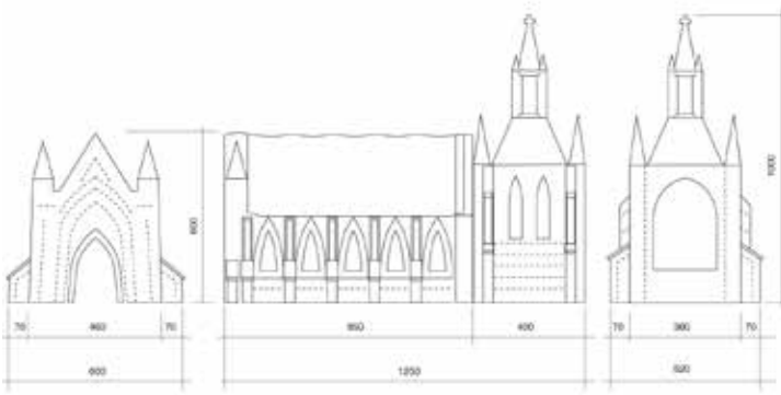
DIMENSIONS INFLATABLE CHURCH - SCALE 1:100 APPROX IN CENTIMETERS
